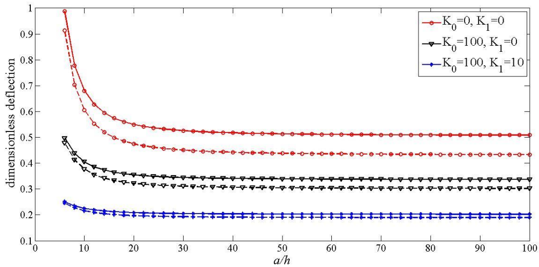
Fig. 2. Variation of dimensionless central deflection \bar{w} of (0^\circ, 90^\circ, 90^\circ, 0^\circ) symmetric (dash lines) and (0^\circ, 90^\circ, 0^\circ, 90^\circ) antisymmetric (solid lines) laminates versus (a/h) ratio for different elastic foundation parameters (material 1).
