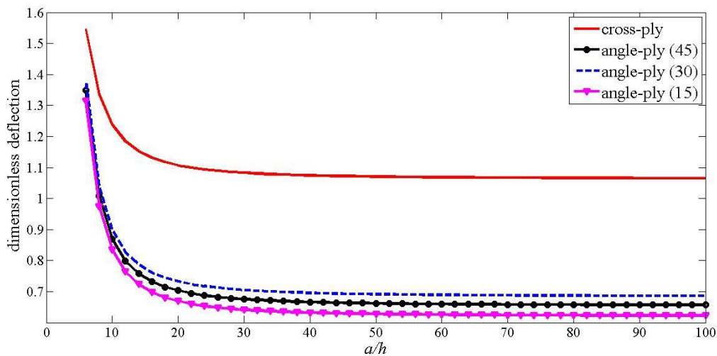
Fig. 3. Variations of dimensionless central deflection of two-layer cross-ply (0^\circ, 90^\circ) and angle-ply (\theta, -\theta) laminates with three different ply-orientation angles versus (a/h) ratio (material 1).
