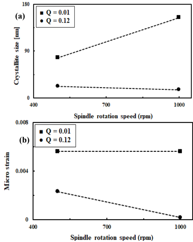
Fig. 4. Interaction plot for machining parameters effects of (a) the crystallite size, (b) and microstrain.
