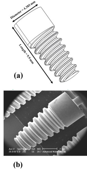
Fig. 1. (a) 3D image of designed implant using SolidWorks software, (b) SEM (Scanning Electron Microscopy) image of the machined implant.
