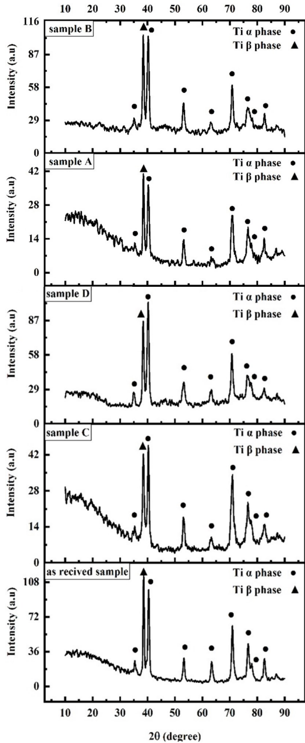
Fig. 2. XRD patterns of as-received, A, B, C, and D samples.
